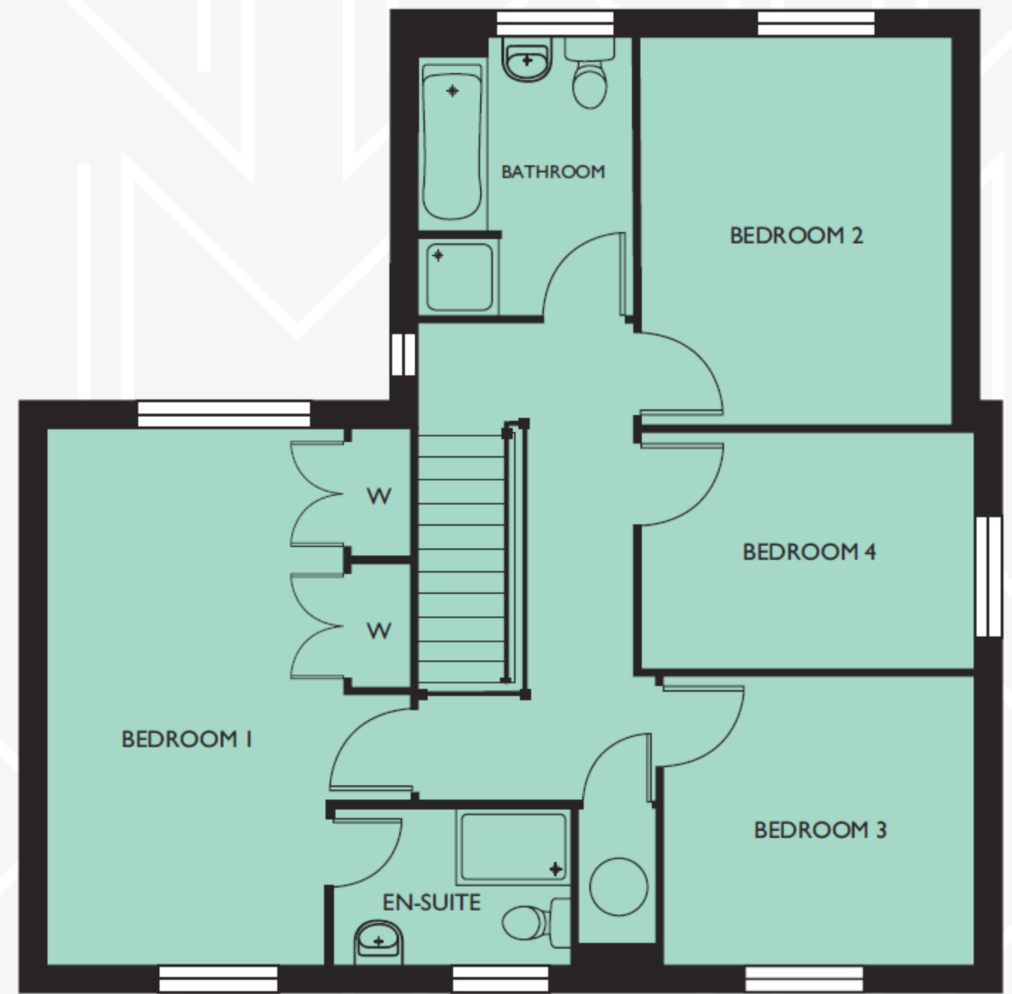
FIRST FLOOR
