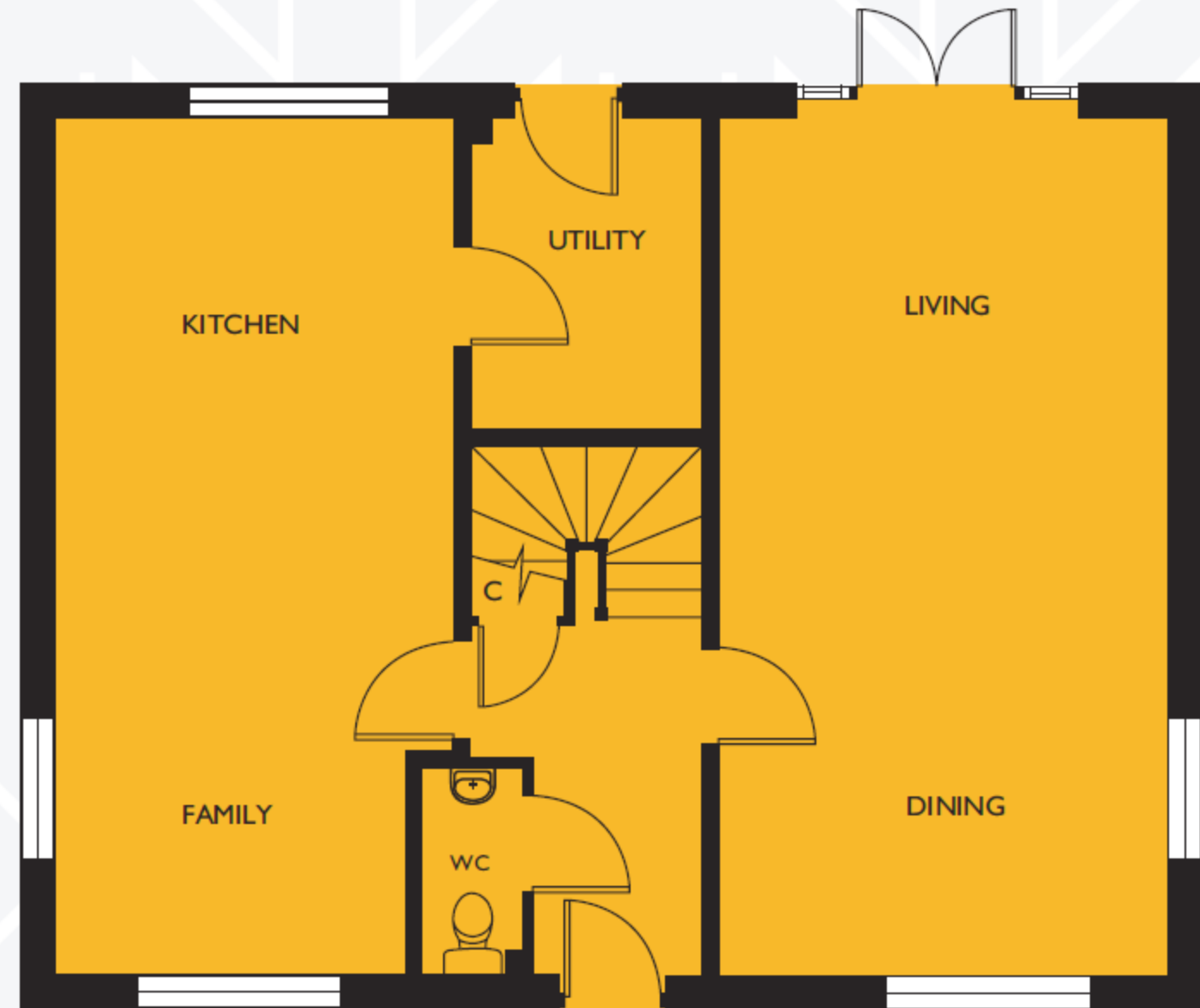
GROUND FLOOR
